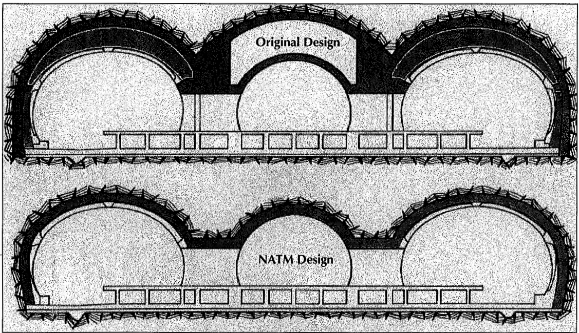
FIGURE 3. Wheaton Station cross sections.
