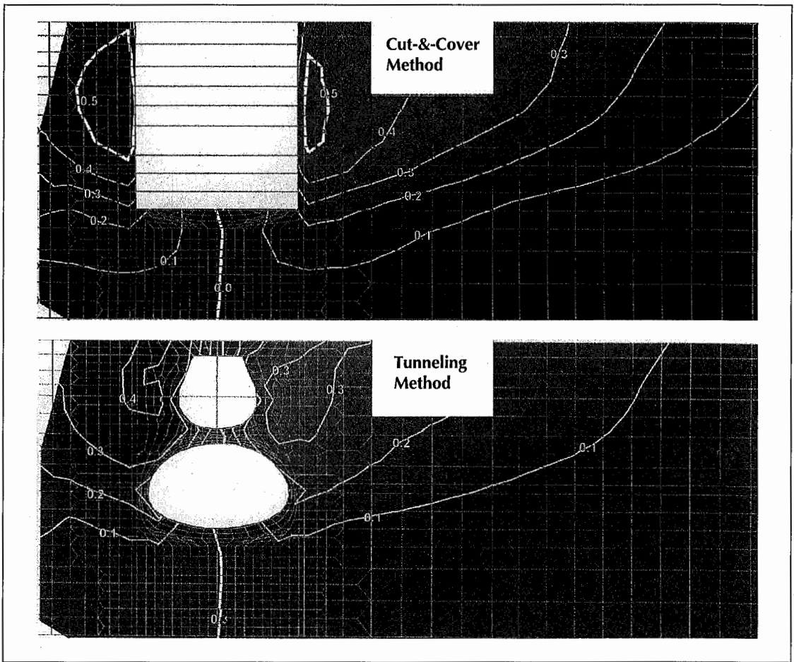
FIGURE 2. Computed horizontal displacements (inches).
