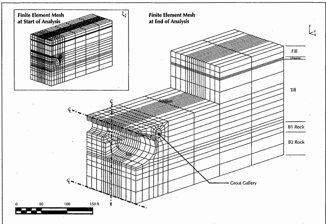
FIGURE 1. Finite element mesh for a tunnel beneath a subway station.
